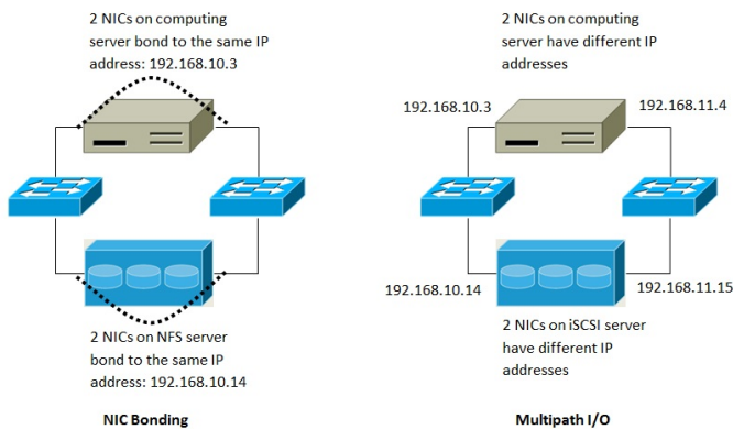
NIC Bonding and Multipath I/O
