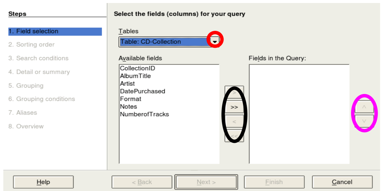
Figure 67: First page of the Query Wizard
