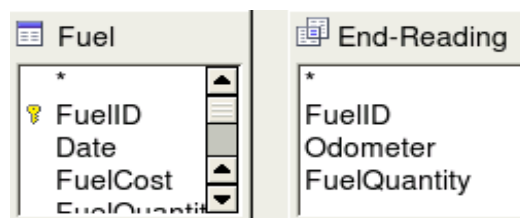
Figure 76: Tables in this query
