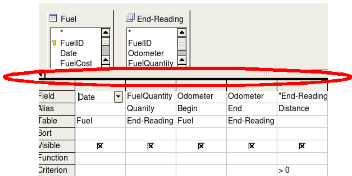
Figure 89: Appearance of query when opened for editing
