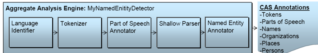
Figure 2.3. Sample Aggregate Analysis Engine
