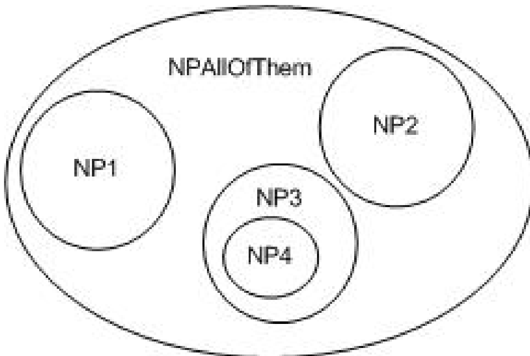
Figure 13.1: Nodepool Example
