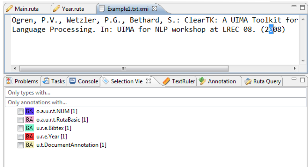
Figure 3.7. Selection view
