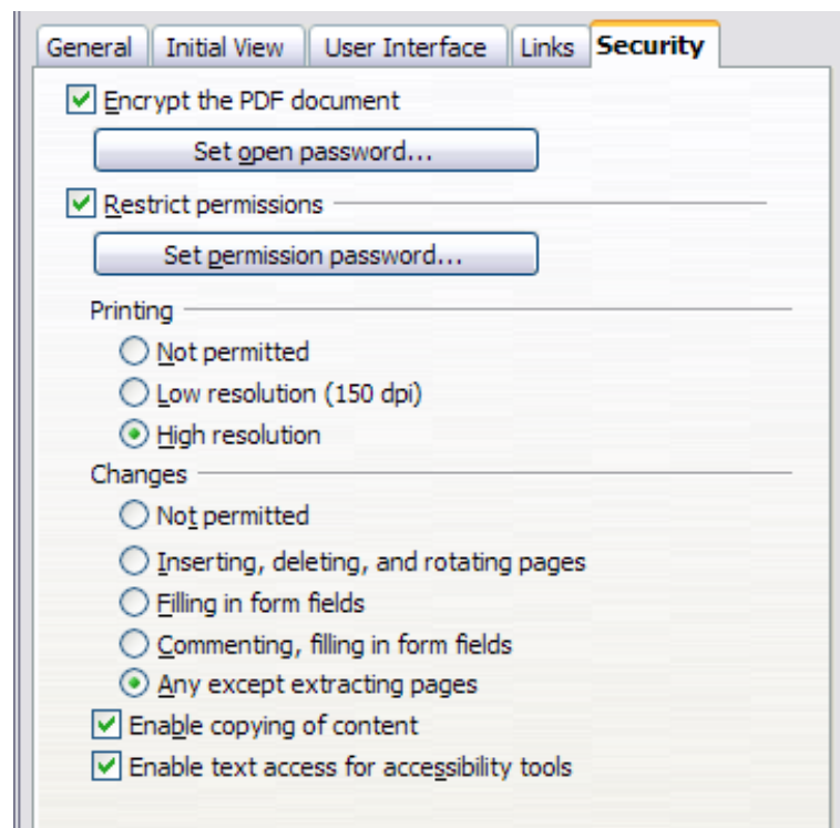
Figure 15: Security page of PDF Options dialog. This dialog is slightly different in OOo3.1, but the functionality is the same.
