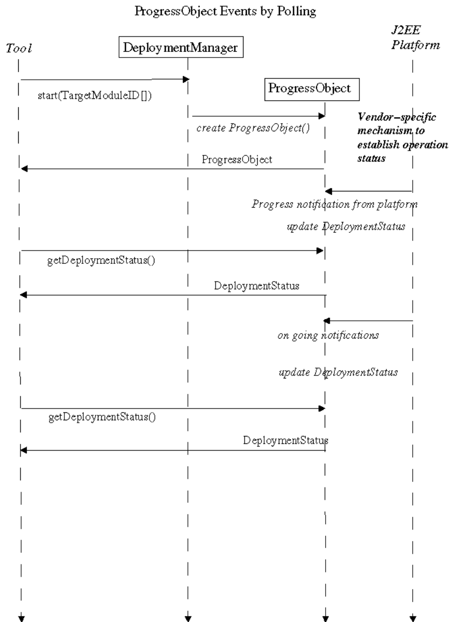
Figure 8.1 ProgressObject Events by Polling
