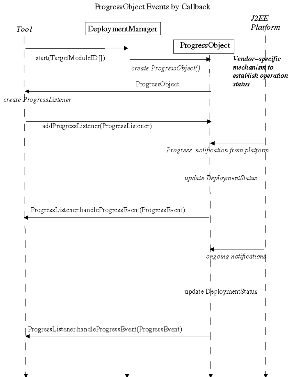
Figure 8.2 ProgressObject Events by Callback
