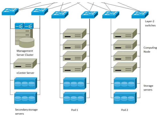
Large-Scale Redundant Deployment
