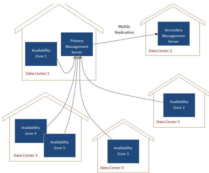
Example of a Multi-Site Deployment
