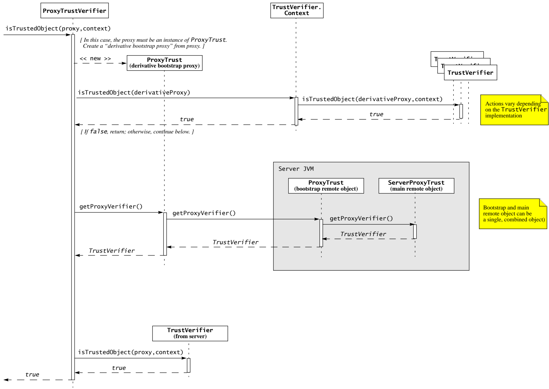
Figure 2: Non-Smart Proxy Trust Verification
